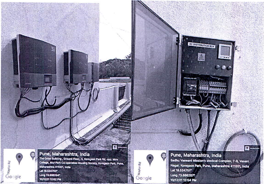
Pic 3 Solar Panel Meter
